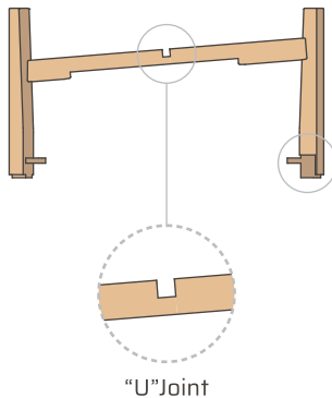
Leg A x 1
