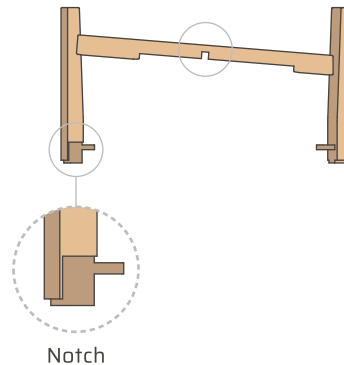
Leg B x 1
