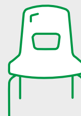
Chairs/arm rests
