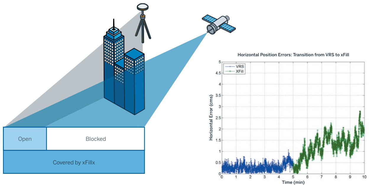
Figure 5. Expected behavior of the Trimble GNSS receiver using Trimble xFill
