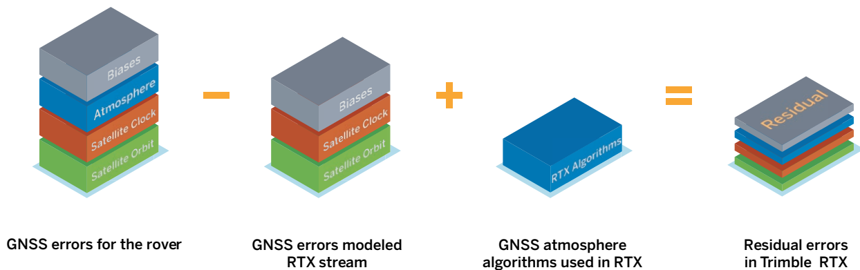
Figure 8. Trimble RTX error modeling
