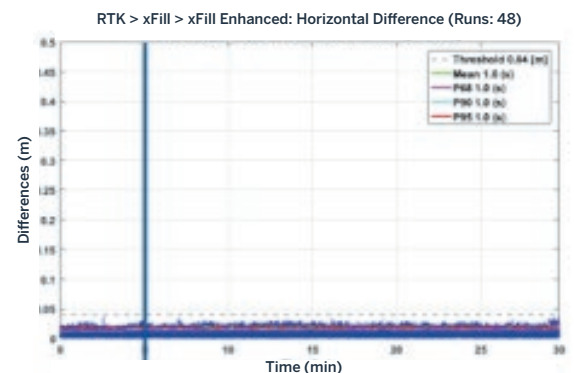
Figure 12. RTK to xFill to xFill Enhanced: example of horizontal difference
