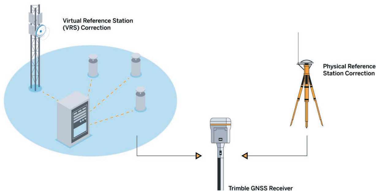
Figure 2. Possible sources of correction for most RTK systems: single physical reference station or VRS
