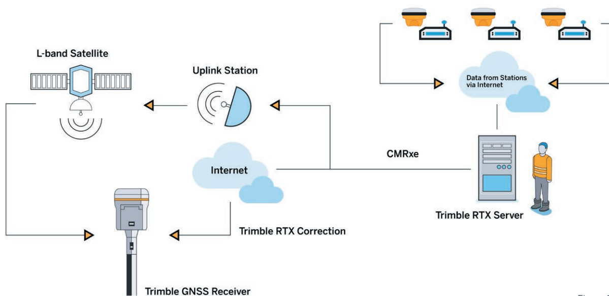
Figure 1. Trimble RTX positioning technology infrastructure
