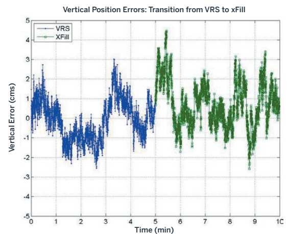
Figure 11. Example of vertical positioning error during extended Trimble xFill
