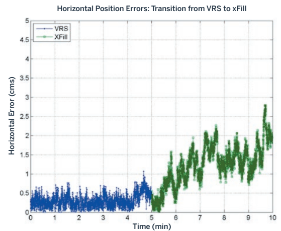
Figure 10. Example of horizontal positioning error during extended Trimble xFill
