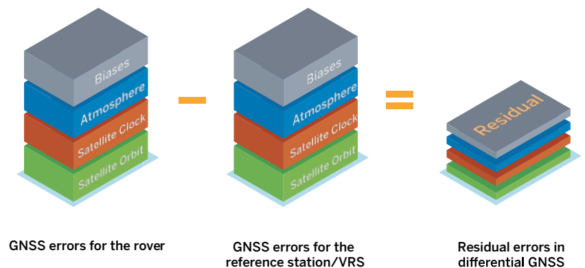
Figure 7. Differential RTK error modeling with single-base or VRS
